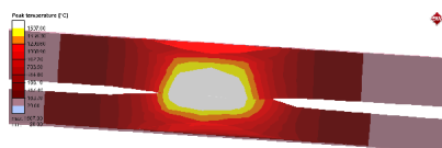
Simufact-GR-thermal-cycle-method.jpg
