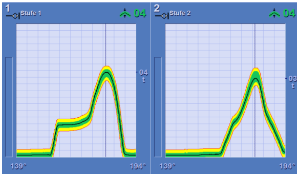
Simufact-GR-Prokos-measured-press-force-distribution.png
