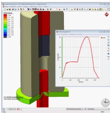
Simufact-GR-Simulationmodel-and-simulated-press-force-distribution-first-station.png
