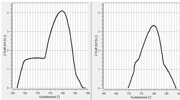
Simufact-GR-simulated-press-force-distribution.png
