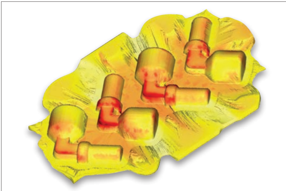
Temperature Profile for the Quadruple Forging of a Brass Elbow
